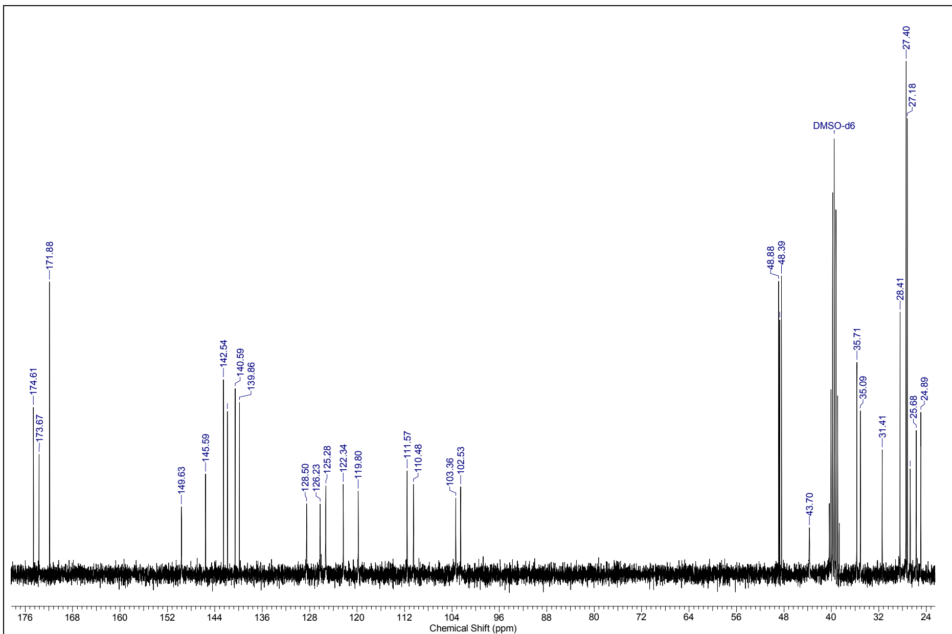
^{13}\text{C} NMR (DMSO- d_6 , 75 MHz)
